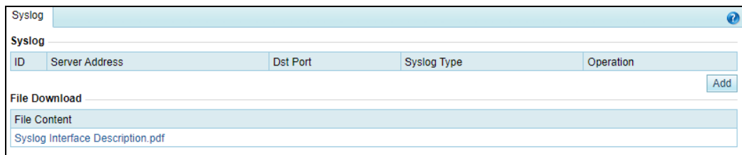
Figure 3-46 Configuring syslog
