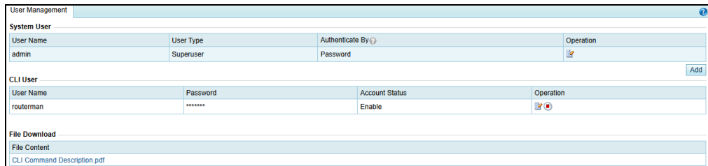
Figure 3-5 System users
