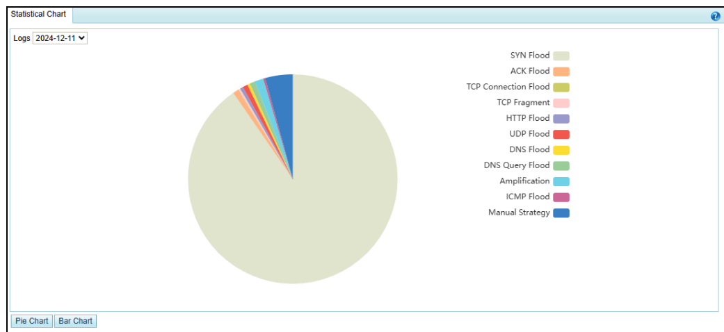
Figure 7-2 Attack proportion
