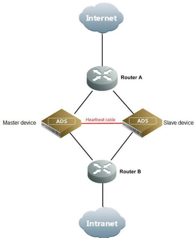
Figure 3-27 Network topology for ADS in in-path mode to implement HA
