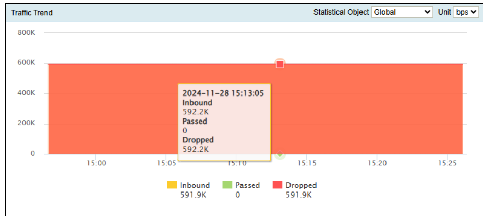
Figure 4-1 Traffic trend
