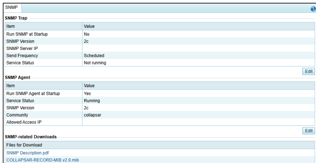
Figure 3-48 SNMP page
