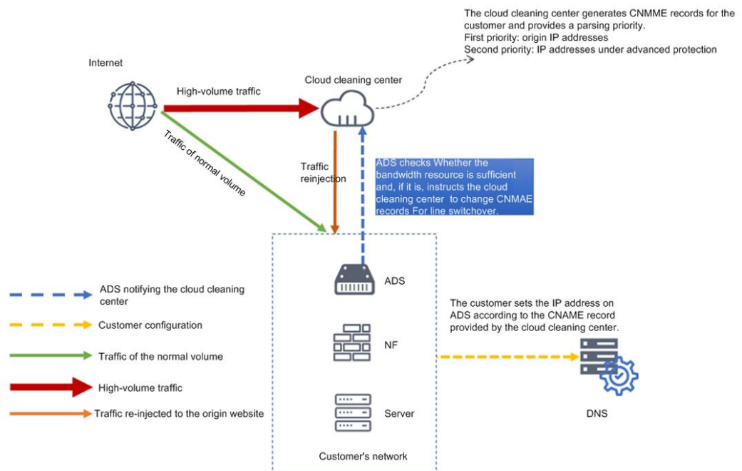
Figure 8-25 Topology of the cloud signaling scenario
