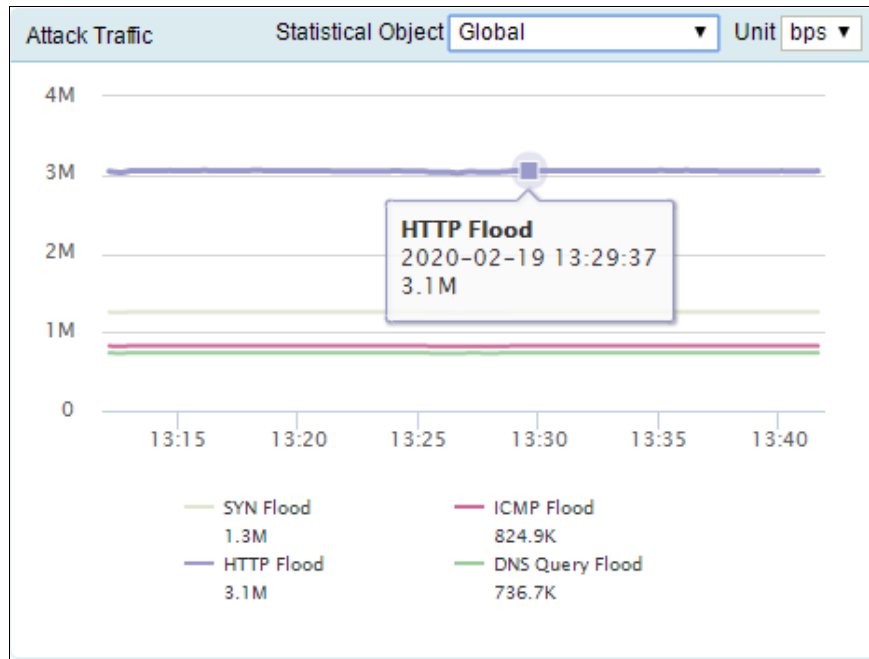
Figure 4-2 Attack traffic
