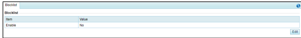
Figure 5-58 Blocklist status
