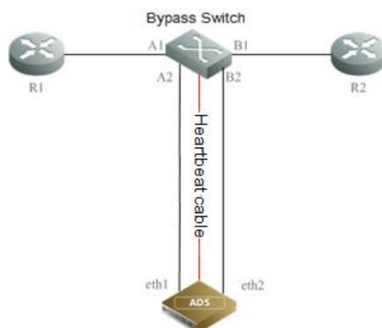
Figure 3-30 Topology for the interaction between ADS and the bypass switch
