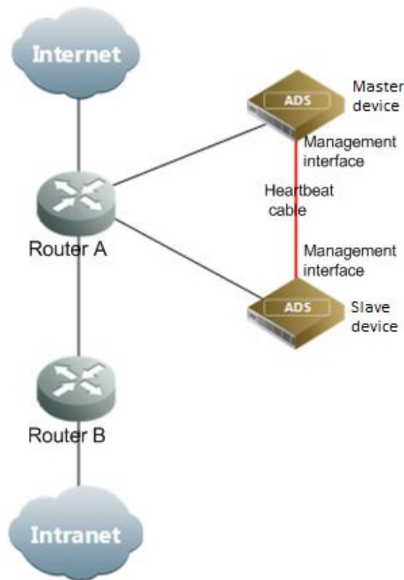
Figure 3-14 Network topology for ADS in out-of-path mode to implement HA
