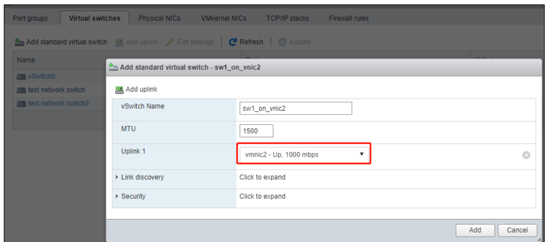
Figure 3-12 Adding a virtual switch
