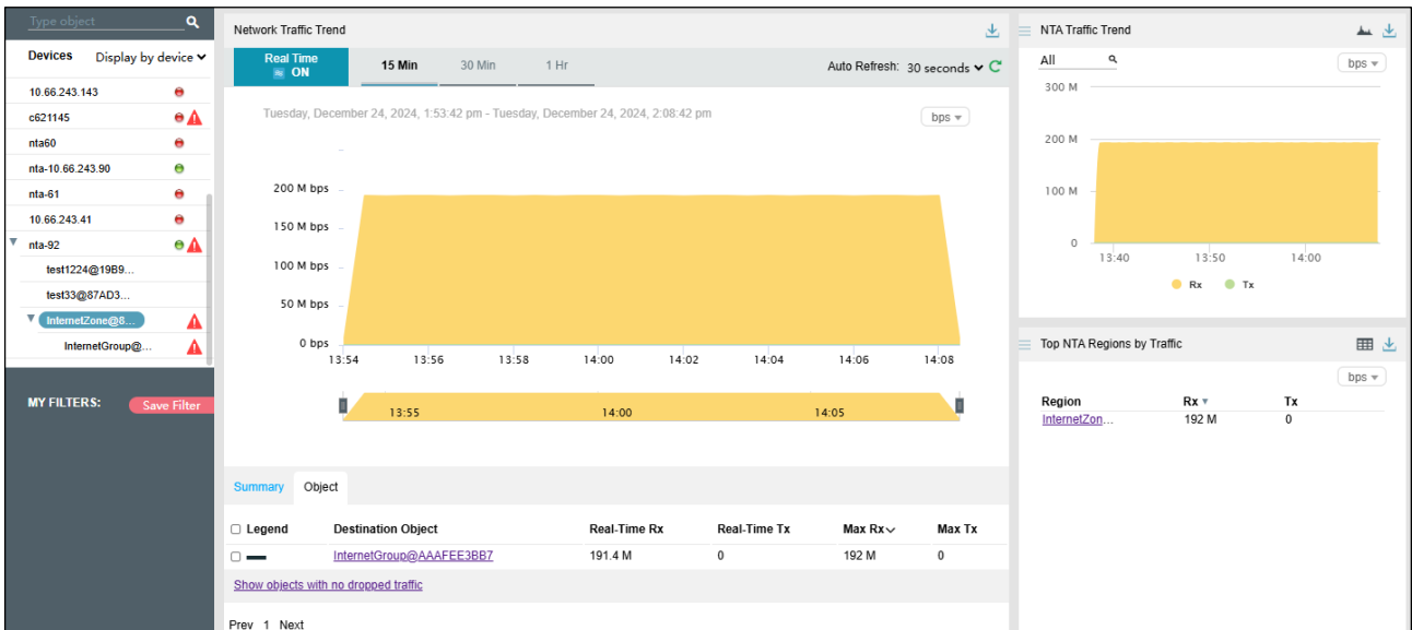
Figure 4-84 Device-specific network traffic information
