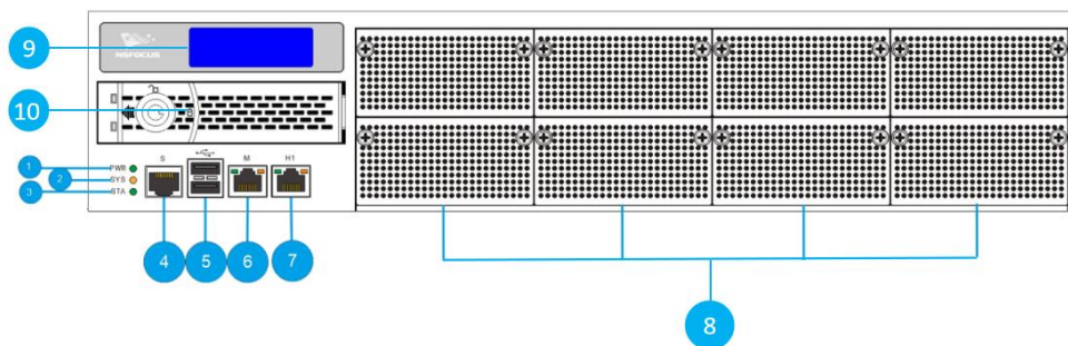
Figure 3-9 Front panel of ADS-M NX3-HD2700
