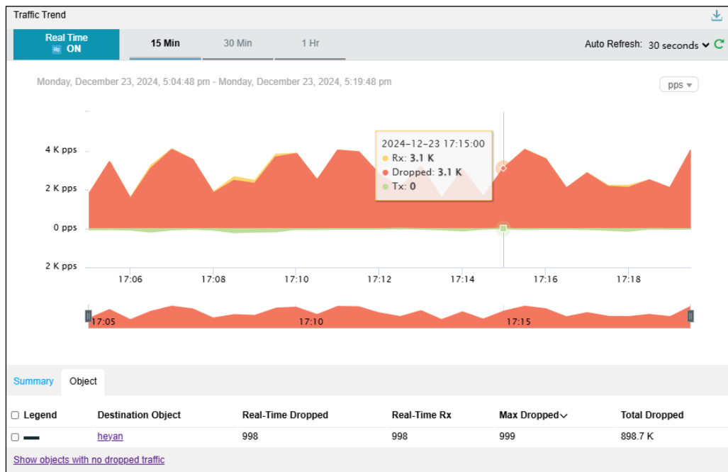
Figure 4-63 Real-time traffic trend graph of a specified object
