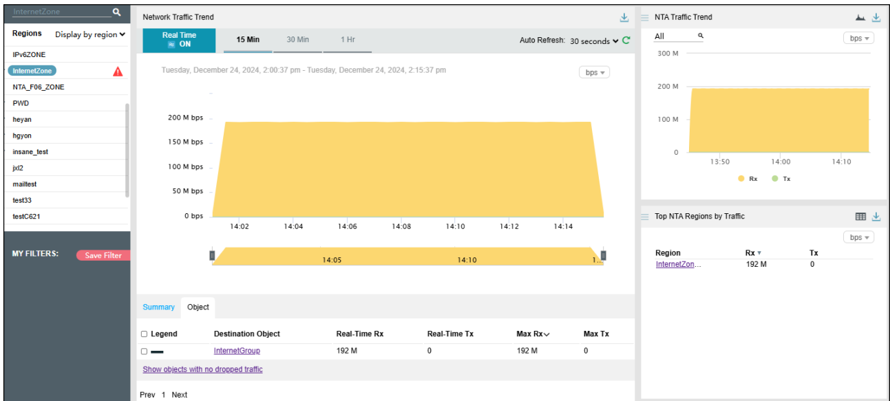
Figure 4-88 Object-specific network traffic information
