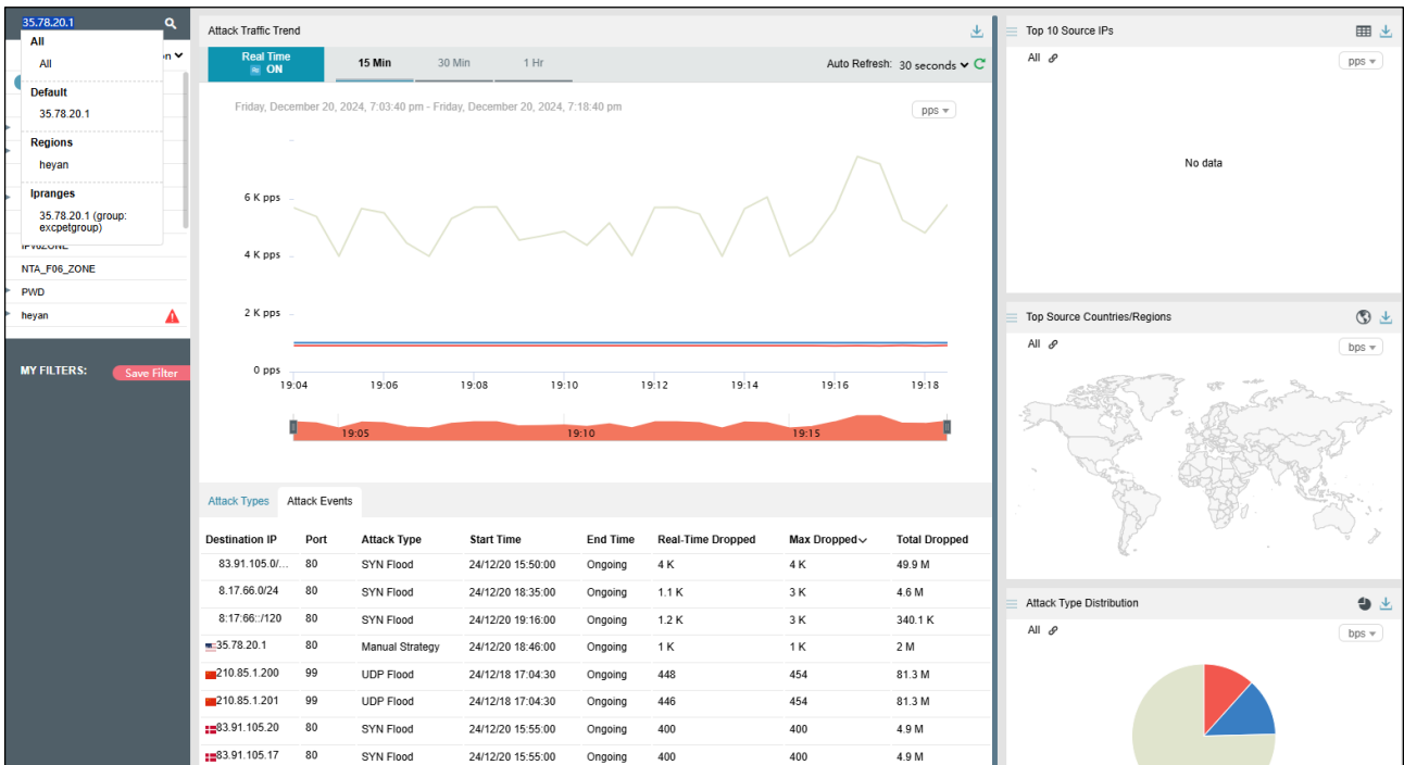
Figure 4-44 Searching for an IP address object
