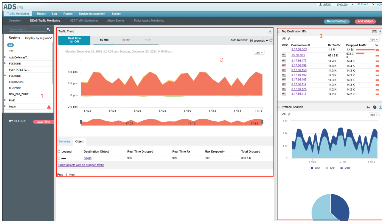
Figure 4-62 Attack traffic information of all objects
