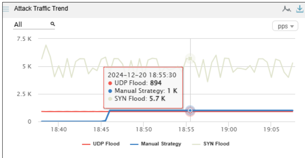
Figure 4-35 Traffic at a specific point of time
