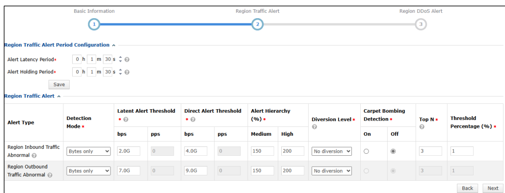
Figure 7-14 Configuring region traffic alert policies
