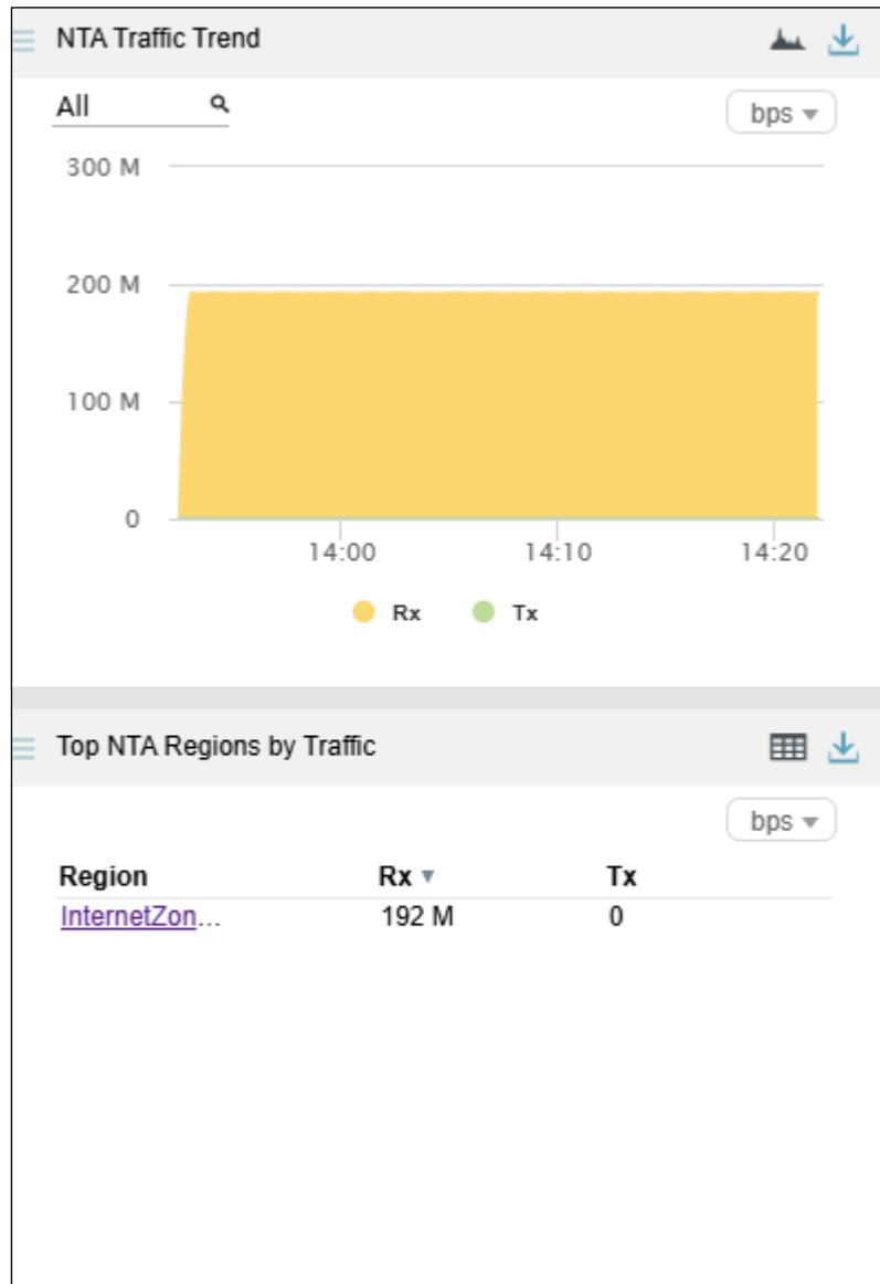
Figure 4-94 Default widgets displayed on the NET Traffic Monitoring page
