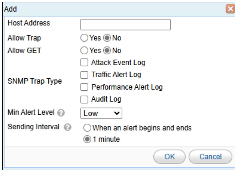
Figure 3-29 Adding an SNMP client
