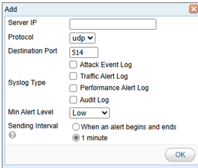
Figure 3-31 Adding a syslog server
