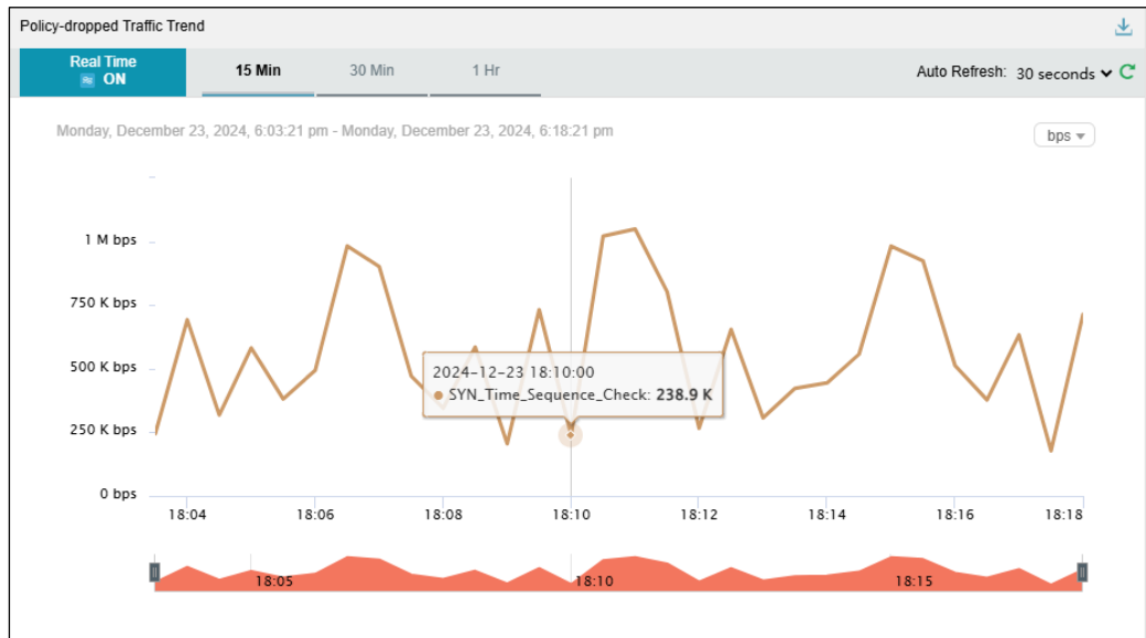
Figure 4-111 Viewing dropped traffic at a specific time
