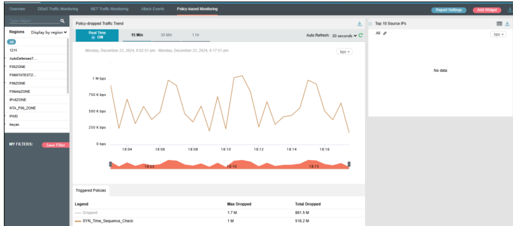
Figure 4-110 Dropped traffic information of all objects
