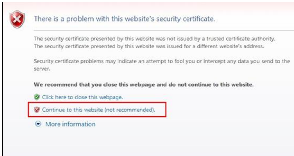
Figure 2-14 Security alert
