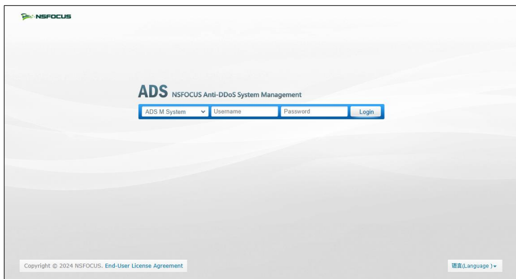
Figure 2-15 Login page
